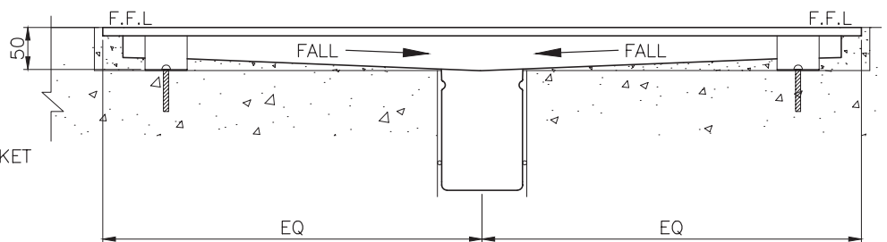
Elevation of typical FT1 floor trough
