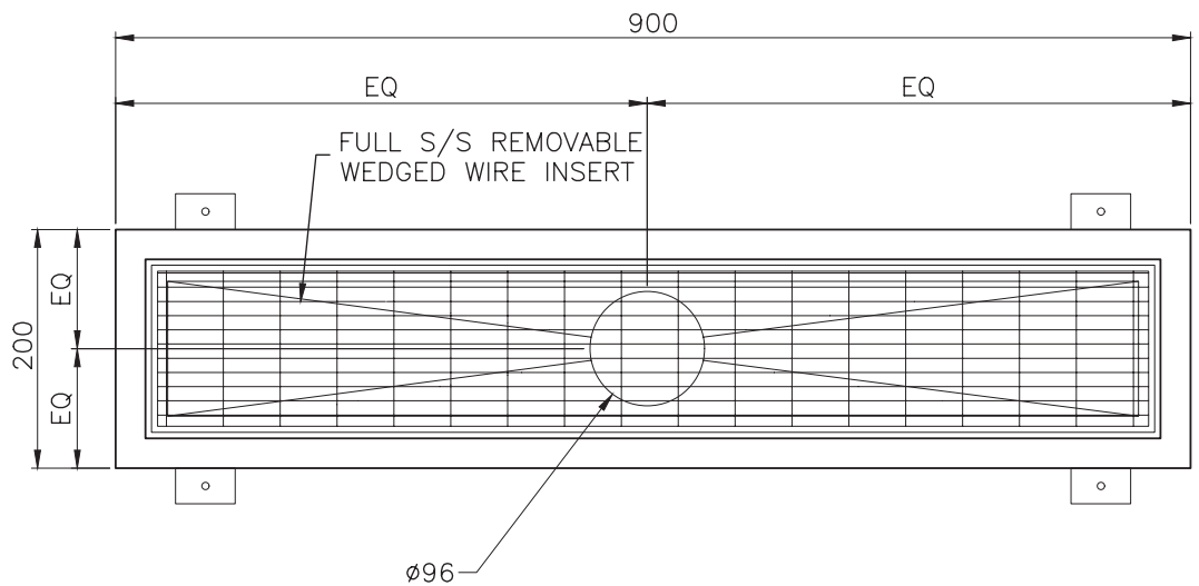
Plan of typical FT1 floor trough
