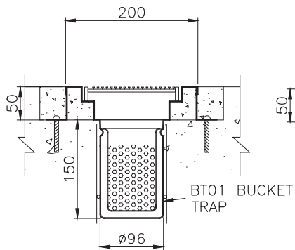
Plan of FT1 bucket trap
