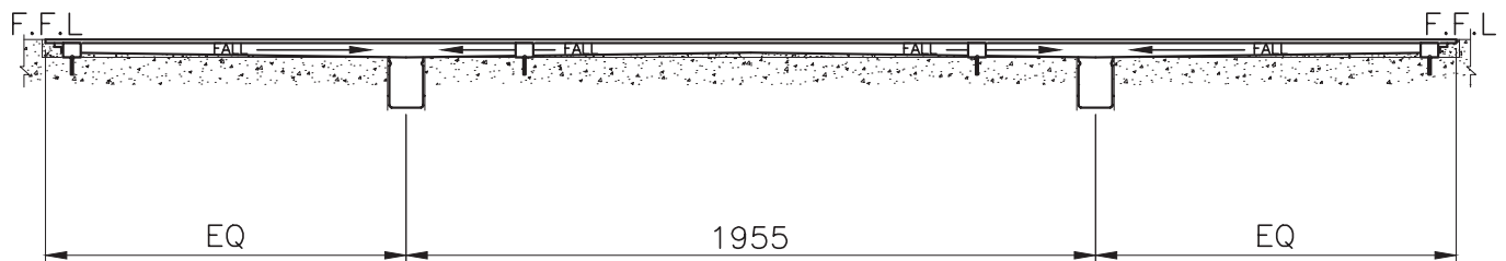
Elevation of typical FT2 floor trough
